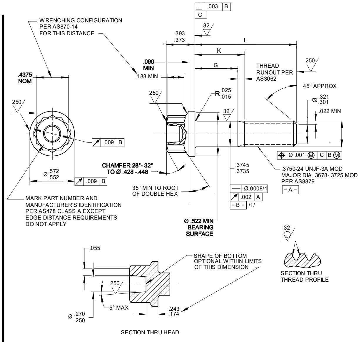
FIGURE 1 - BOLT
